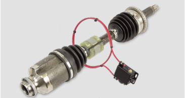
Shaft Instrumentation with Slip Ring or Telemetry (2)
