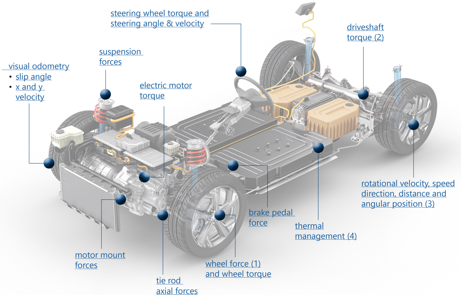
Wheel Force Transducer (1)
