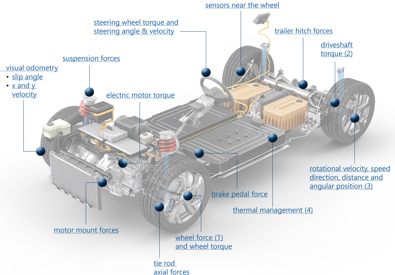
Wheel Force Transducer (1)
