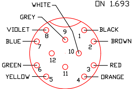
FRONT VIEW OF STATOR CONNECTOR ON SLIP RING. COLORS OF STATOR CABLE WIRES & ROTOR WIRES.
